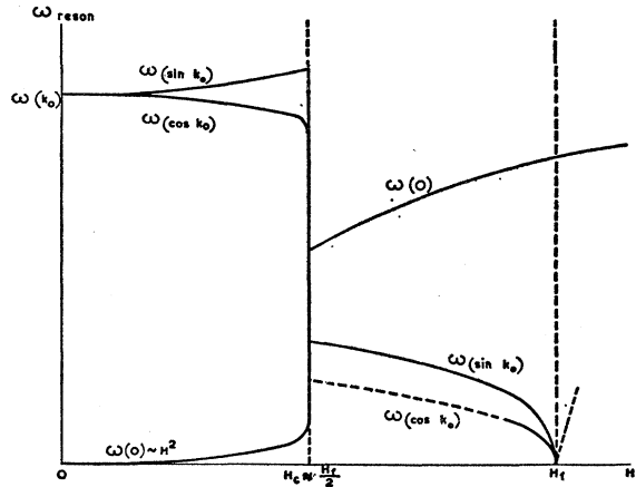
FIG. 1. Variation of resonance frequencies with applied field for the case of zero planar anisotropy. (The resonances can be excited only for values of H where the variation is indicated by a solid line.)
